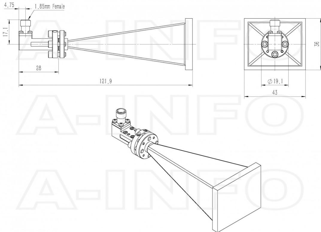
1.85mm-Female Output with Radome (Option, P/N: LB-15-25-C-1.85FSPO, Outdoor Application)
